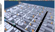
Rhode Island night club fire simulation: 800K contour; comparison of experiment and SMARTFIRE prediction showing combusting surfaces
